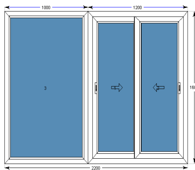
Fix + 2 Track Sliding
