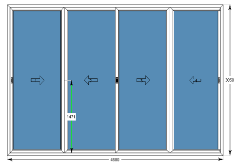
2x 4 Panel Sliding System
