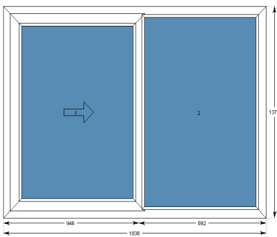
Fix + 1-Track Sliding Window
