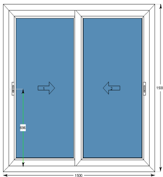
2-Track Sliding Window
